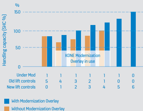
Group handling capacity with and without Modernization Overlay in destination control system modernization
